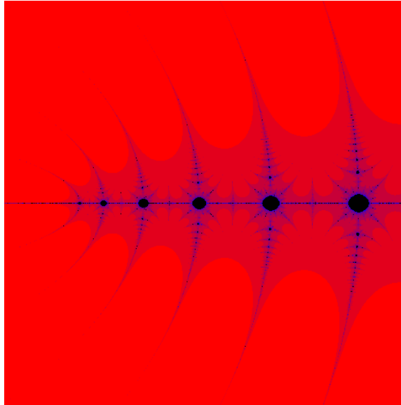
Figure 2.3: Julia Set of C_{40.77235+.00007i,0} , with -400 \leq \text{Re}(z) \leq 2000 and |\text{Im}(z)| \leq 1200
