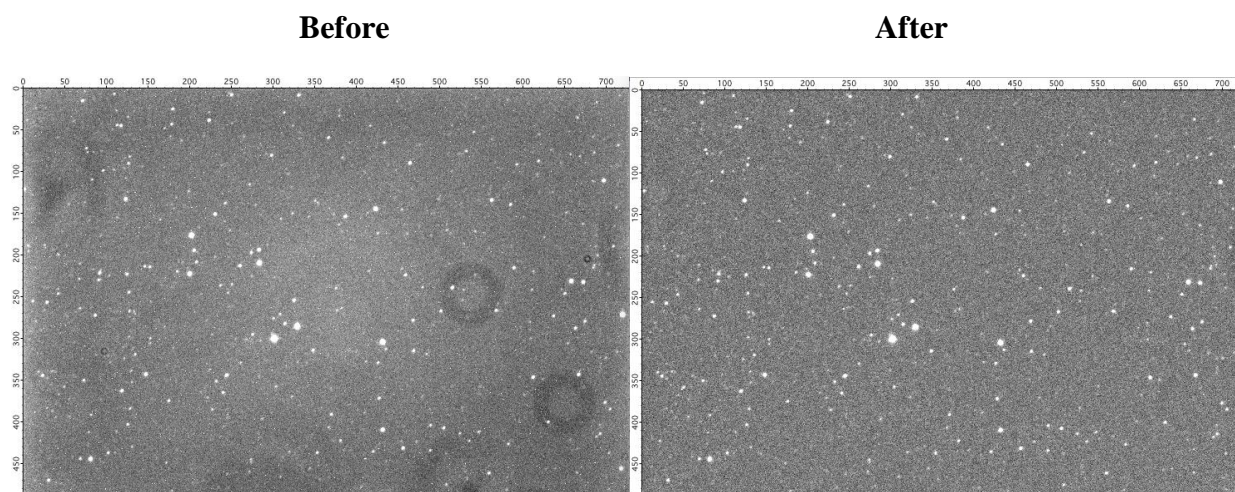
Figure 3: The sky in the R-filter.
