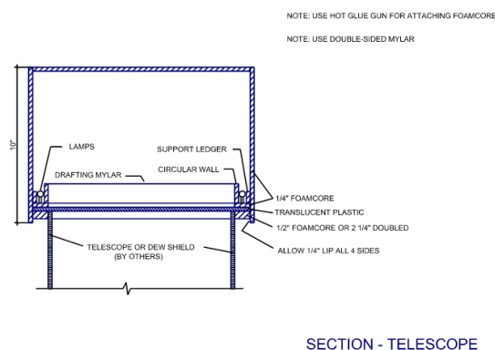
Figure 1: Example schematic of a lightbox ( http://www.gregpyros.com/assets/Lightbox-pyros.pdf )
